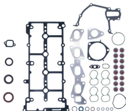
Full Gasket Set without Cylinder Head Gasket OEM No: 71769851S Avortex No: 381
