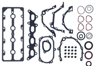
Full Gasket Set without Cylinder Head Gasket OEM No: 71716871 Avortex No: 2800S
