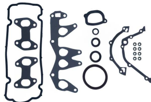
Full Gasket Set without Cylinder Head Gasket OEM No: 5893663 Avortex No: 2700S
