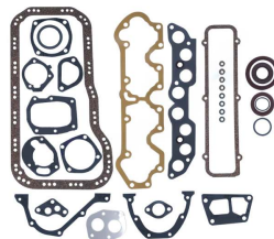
Full Gasket Set without Cylinder Head Gasket OEM No: 71737118F Avortex No: 3200S
