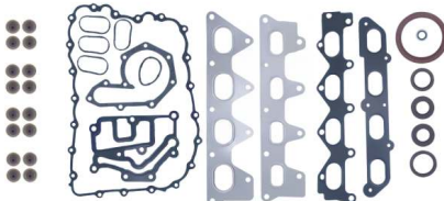
Full Gasket Set without Cylinder Head Gasket OEM No: 7701471278F Avortex No: 5800S
