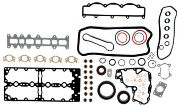
Full Gasket Set without Cylinder Head Gasket OEM No: 504049360 Avortex No: 600
