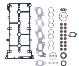
Cylinder Head Gasket Set without Cylinder Head G... OEM No: 71769851 Avortex No: 384
