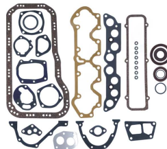
Full Gasket Set without Cylinder Head Gasket OEM No: 71737120F Avortex No: 3300S
