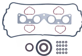
Full Gasket Set without Cylinder Head Gasket OEM No: 7701475822 Avortex No: 4590S
